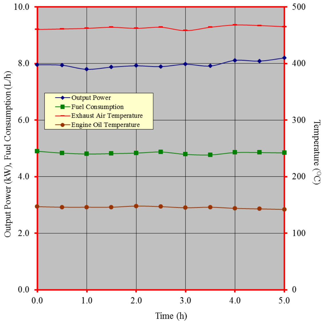
Figure 4. Performance characteristic curves during the continuous running test of the DUCAR DJ190F gasoline engine
