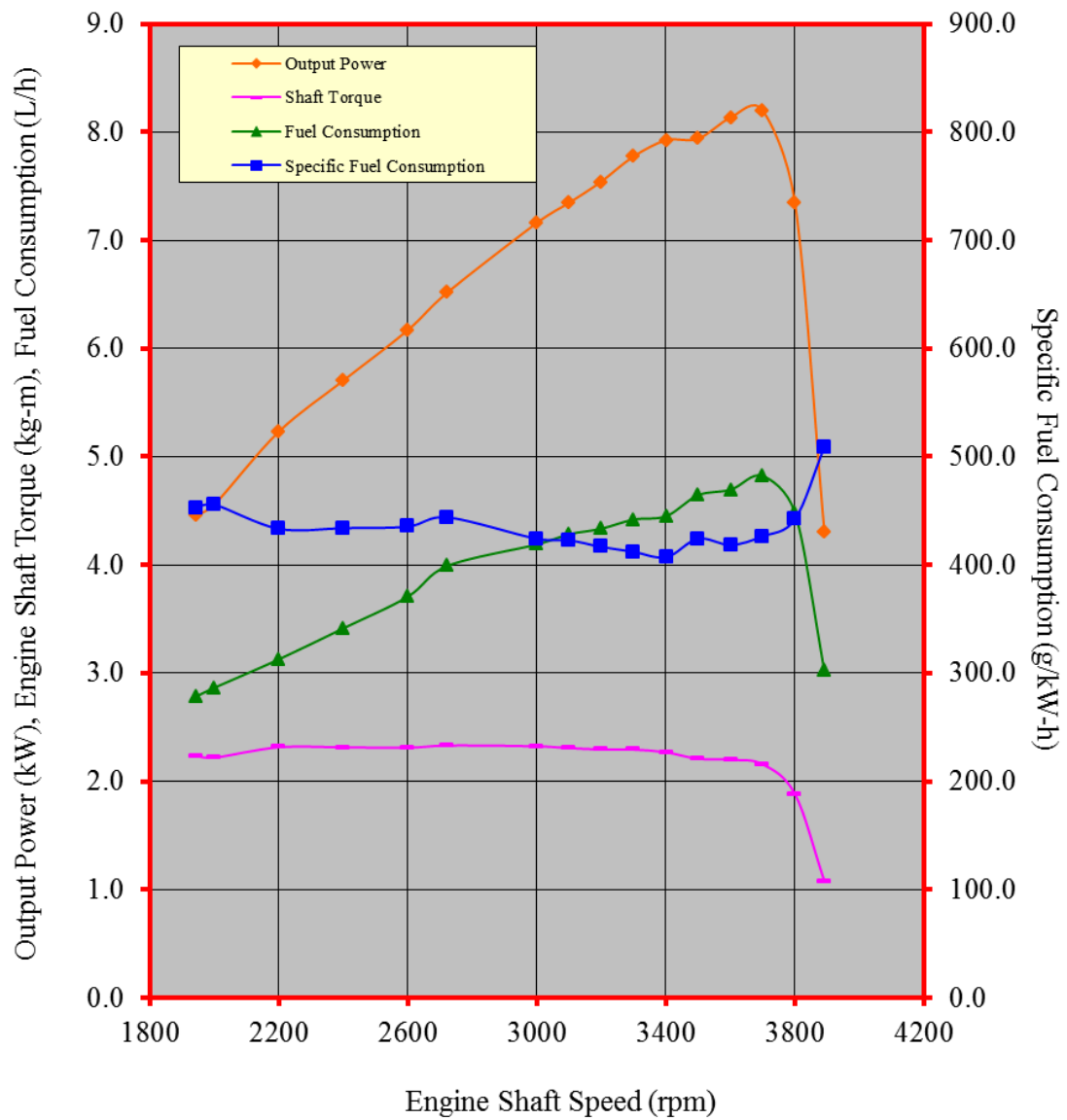
Figure 3. Performance characteristic curves of the DUCAR DJ190F gasoline engine
